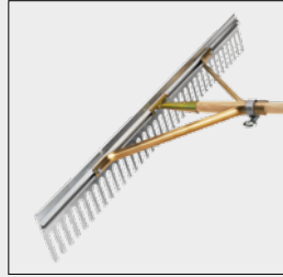
Strong struts stabilise the wide aluminium rake and the pull-off profile.
